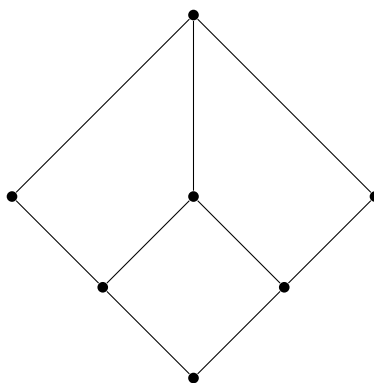
FIGURE 3. The lattice L_7
